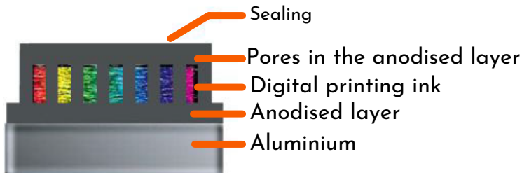
Schematic structure/cross-section of an aluminium plate
